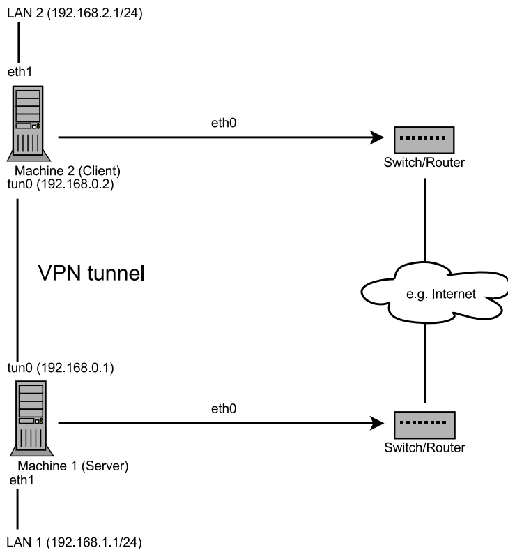
Figure 15.1 Routed VPN
