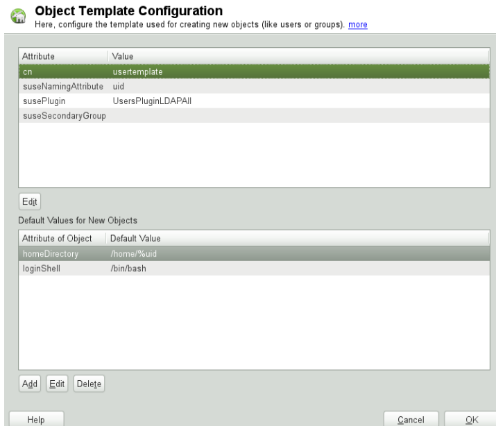
Figure 4.9 YaST: Configuration of an Object Template
