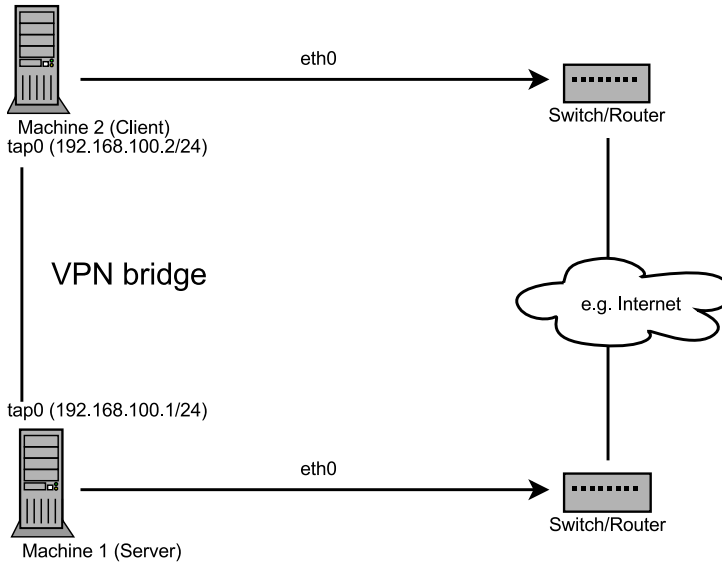
Figure 15.3 Bridged VPN - Scenario 2
