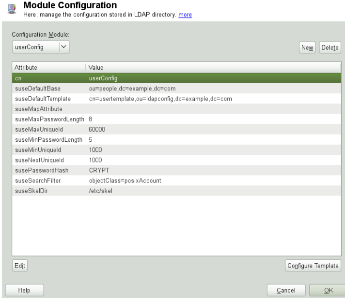
Figure 4.8 YaST: Module Configuration
