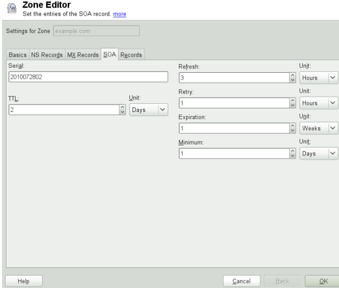
Figure 25.8 DNS Server: Zone Editor (SOA)
