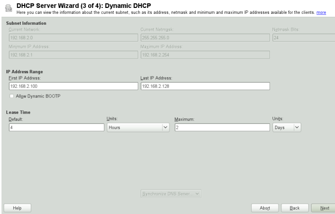
Figure 26.3 DHCP Server: Dynamic DHCP
