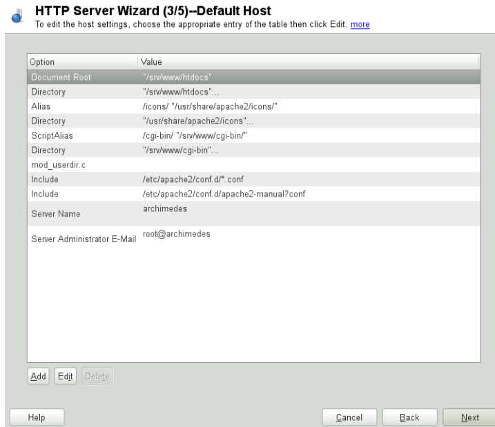
Figure 30.1 HTTP Server Wizard: Default Host
